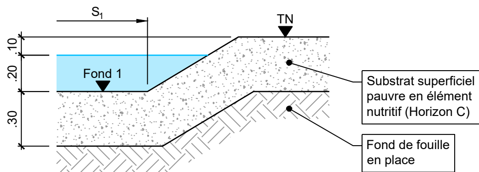
Coupe A - A 1:20 [m]
